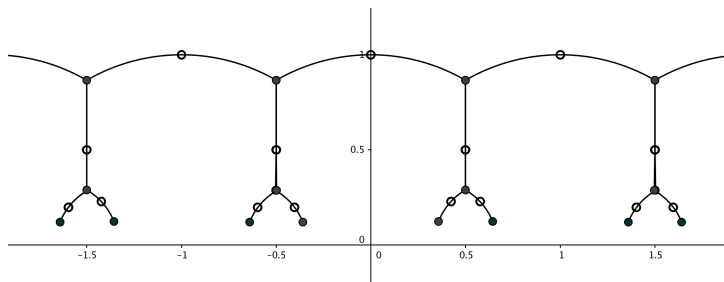
FIGURE 1. The Farey tree, \mathcal{F} .
